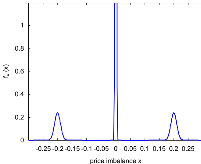
Fig. 5. Density of idiosyncratic shocks.
