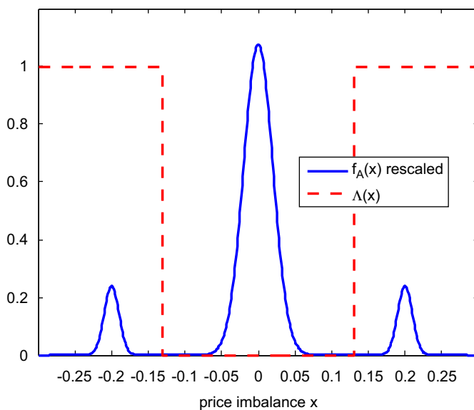
Fig. 6. Ergodic density and Ss bands.
