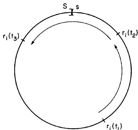
Fig. 1. The Caplin and Spulber model.
